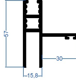
Tek Cam Fitilli & Kenetli Kanat
