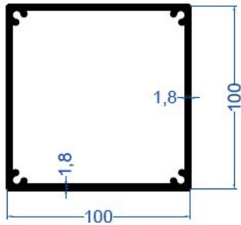
Kutu Profili 100X100
