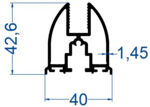
"Gold" Kanat Profili
