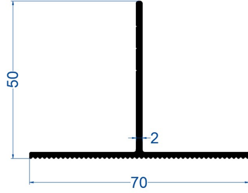
50*70*2,0 mm "T" Profil
