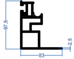
E-1017 3,009 kg/m Alt Ray Profili
