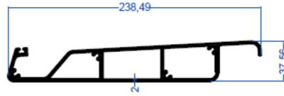
E-1440 3,415 kg/m Panel Profili
